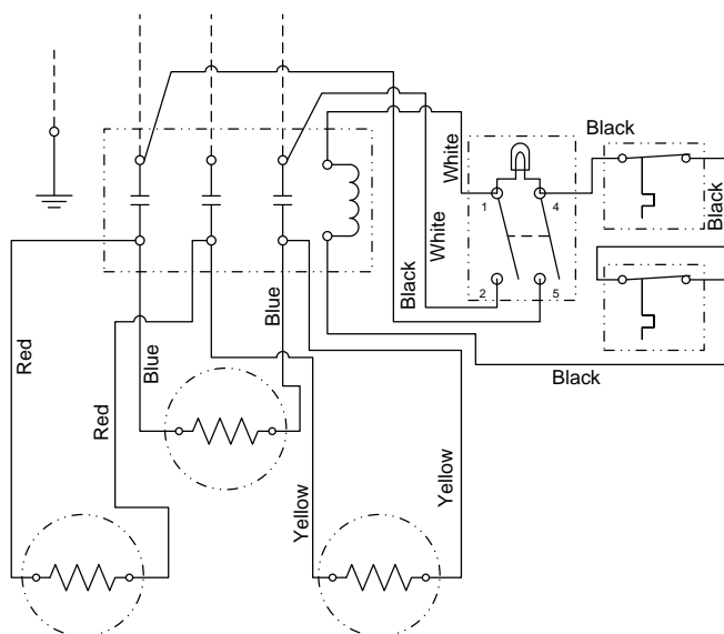
3-Phase
