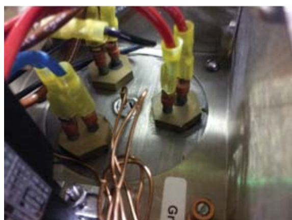
The three heater elements located behind hi-limit
