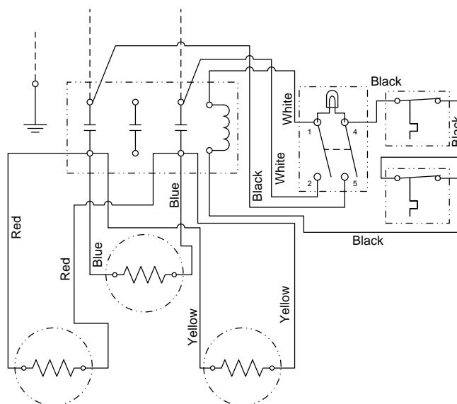
Single Phase
